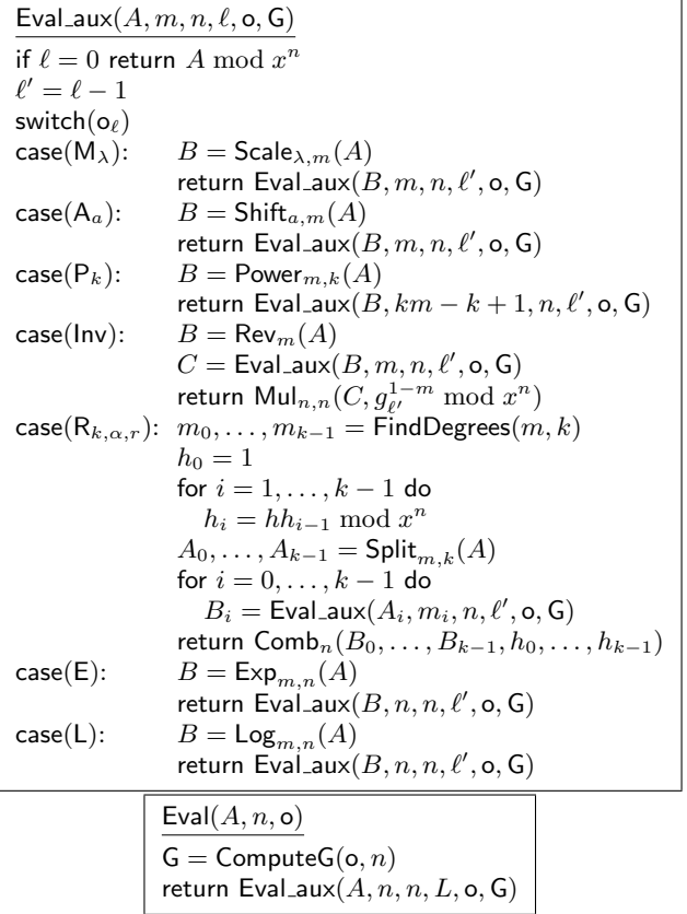
Figure 1: Algorithm Eval.
