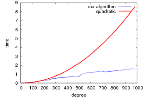
Figure 4: Mittag-Leffler polynomials.
