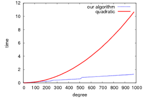
Figure 3: Jacobi polynomials.
