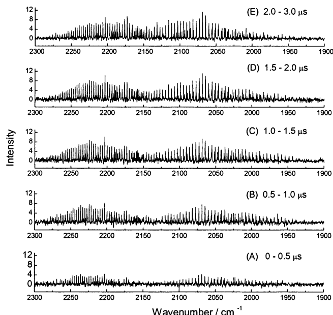
Figure 1. Infrared emission spectra of CO in the spectral region 2300–1900 cm ^{-1} averaged for periods 0–0.5 (A), 0.5–1.0 (B), 1.0–1.5 (C), 1.5–2.0 (D), and 2.0–3.0 \mu s (E) after photolysis of (ClCO) 2 at 0.056 Torr and 298 K with a KrF laser at 248 nm. Resolution is 0.3 cm ^{-1} ; 70 laser pulses were averaged at each scan step. Four spectra recorded under similar conditions were averaged.
