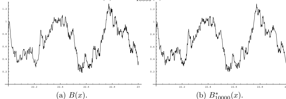
FIGURE 2. B(x) and B_{10000}^*(x) for 22 \leq x \leq 23 .
