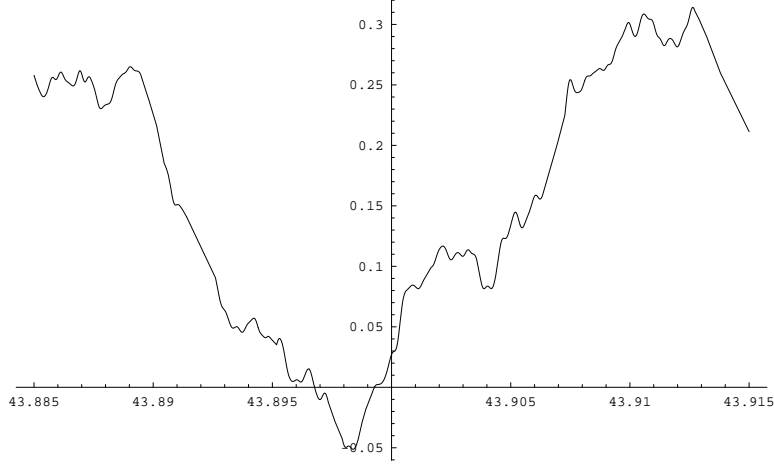
FIGURE 4. B_{25000}^*(x) near x = 43.9 .
