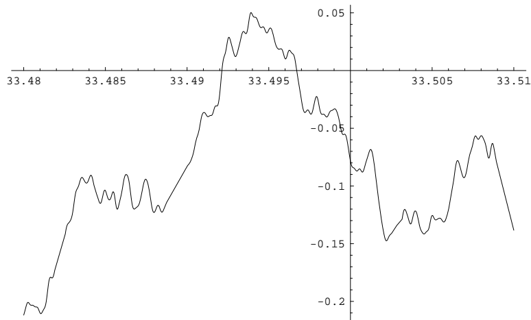
FIGURE 5. A_{25000}^*(x) near x = 33.5 .
