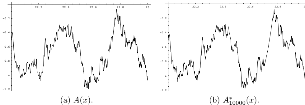
FIGURE 1. A(x) and A_{10000}^*(x) for 22 \leq x \leq 23 .
