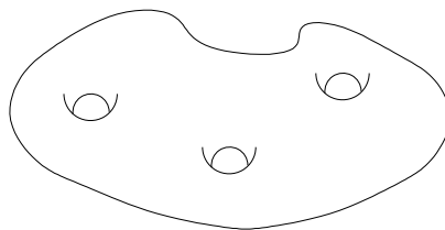
FIGURE 18.1. A genus 3 Riemann surface
