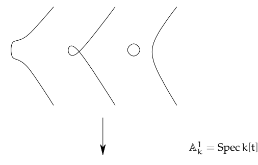
FIGURE 24.1. A flat family of smooth curves degenerating to a nodal curve: y^2 = x^3 + x^2 + tx .
