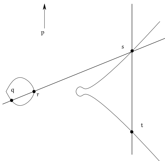
FIGURE 19.4. The group law on the elliptic curve, geometrically
