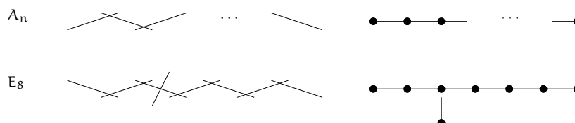
FIGURE 22.2. The exceptional divisors for resolutions of some ADE surface singularities, and their corresponding dual graphs (see Remark 22.4.5)
