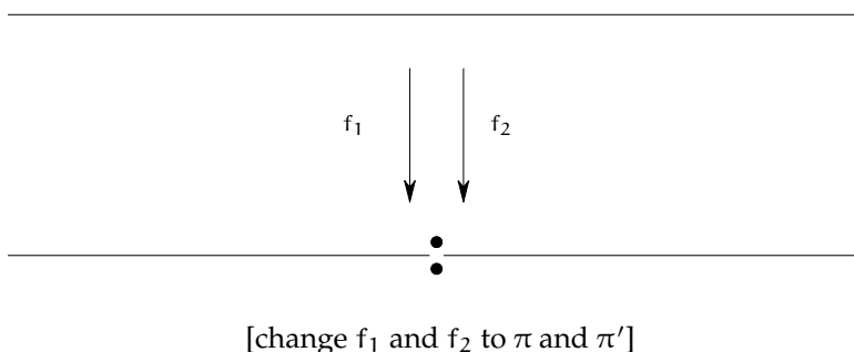
FIGURE 10.5. Two different maps to a nonseparated scheme agreeing on a dense open set
