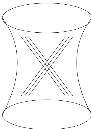
FIGURE 8.2. The two rulings on the quadric surface V(wz - xy) \subset \mathbb{P}^3 . One ruling contains the line V(w, x) and the other contains the line V(w, y) .
